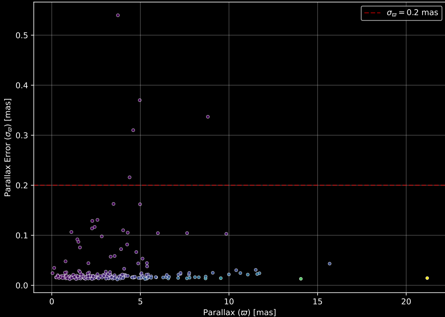
APOGEE DR17 Field: [185-42_MGA] Parallax Quality (n= 223)
