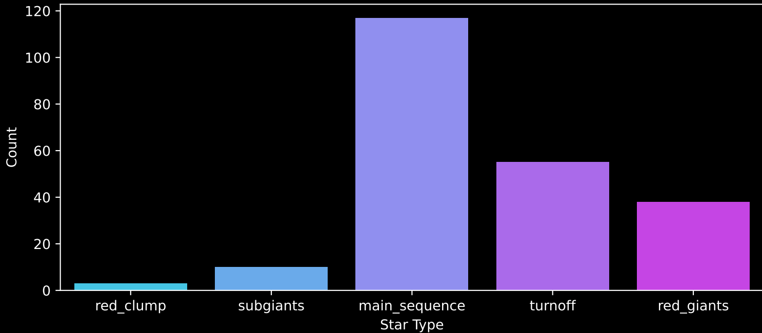
APOGEE DR17 Field: [185-42_MGA] Count plot of Star Type
