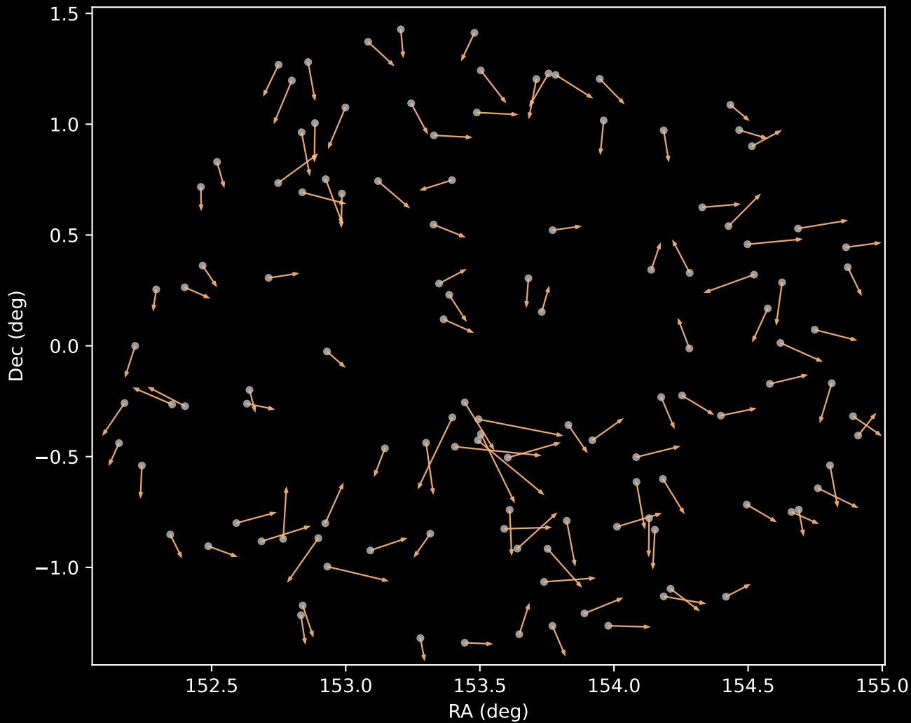
APOGEE DR17 Cluster 3 Proper Motion Vectors (n=120)
