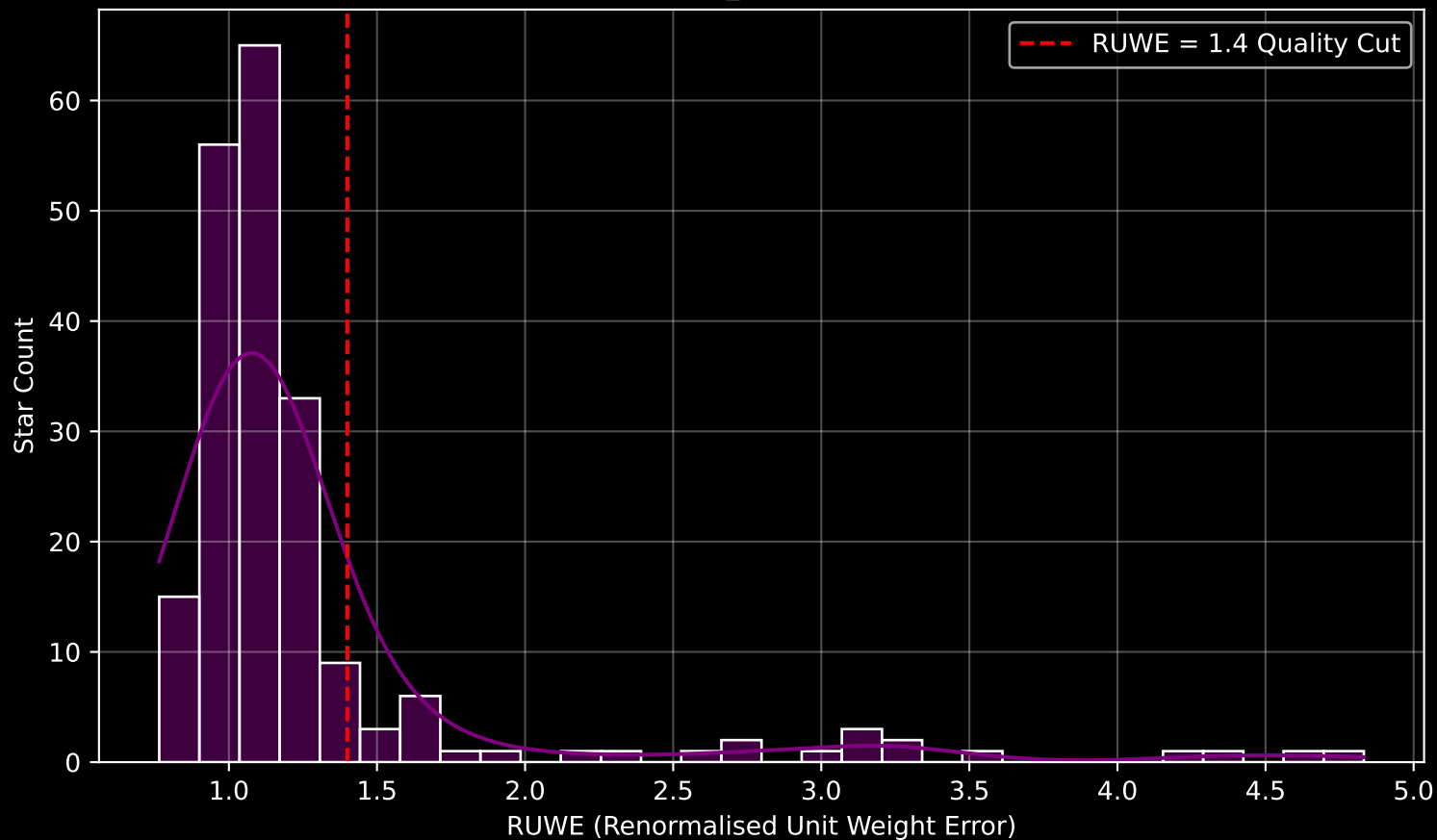
GAPOGEE DR17 Field [185-42_MGA] RUWE Distribution (n= 205)
