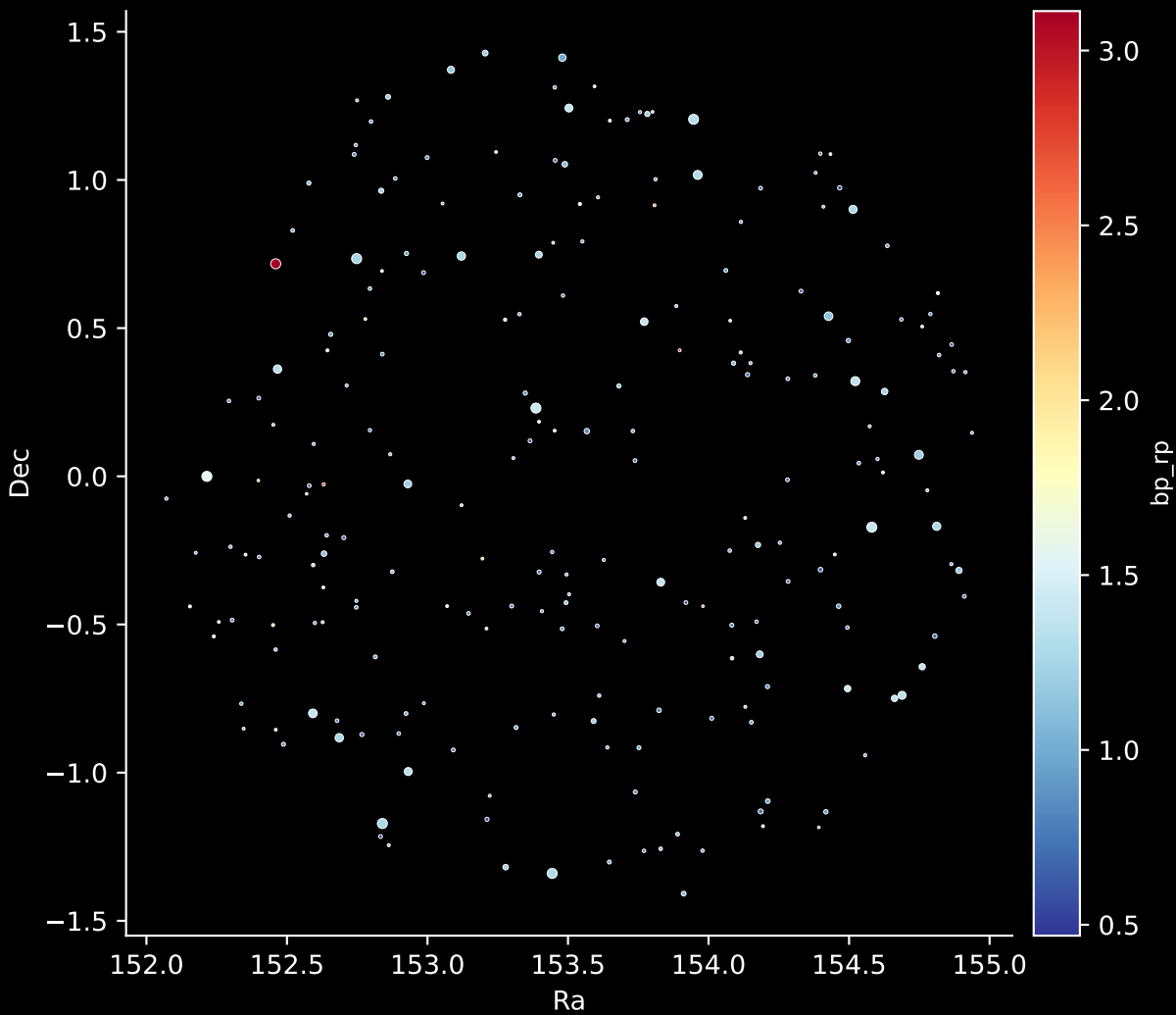
APOGEE DR17 Field: [185-42_MGA] Stars: 223
