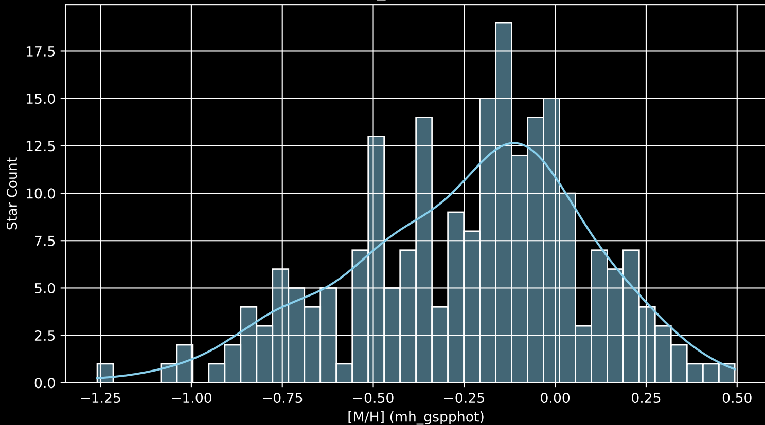
APOGEE DR17 Field: [185-42_MGA [M/H] (mh_gspphot) (n= 222)
