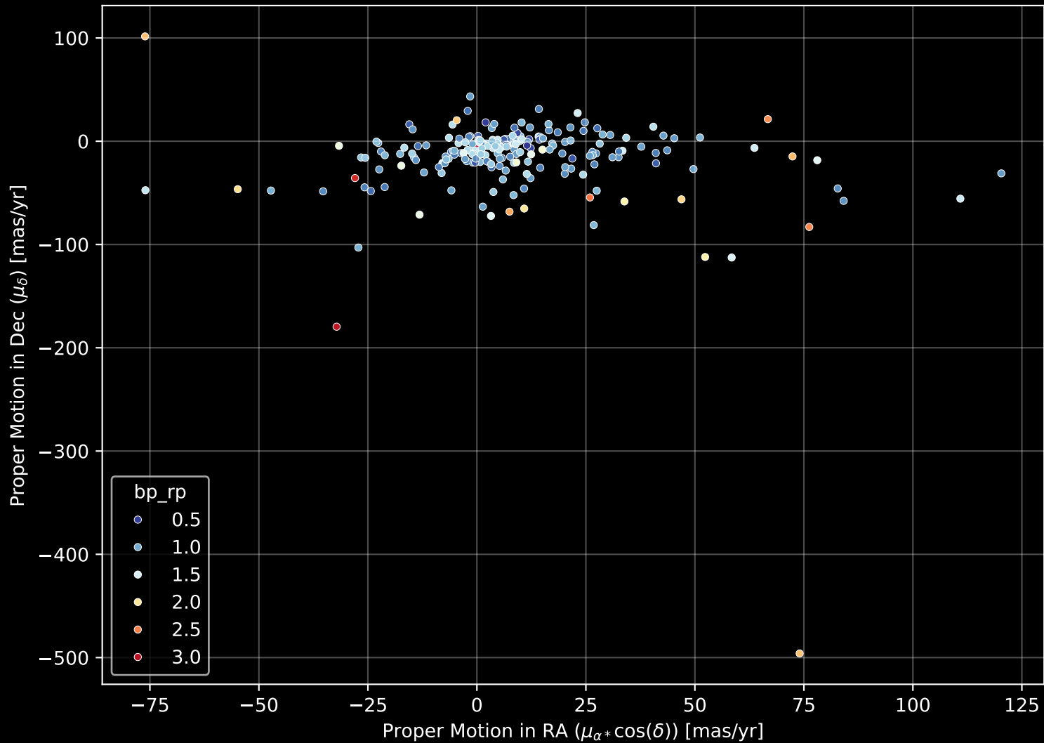
APOGEE DR17 Field: [185-42_MGA] Proper Motion Diagram (n= 223)
